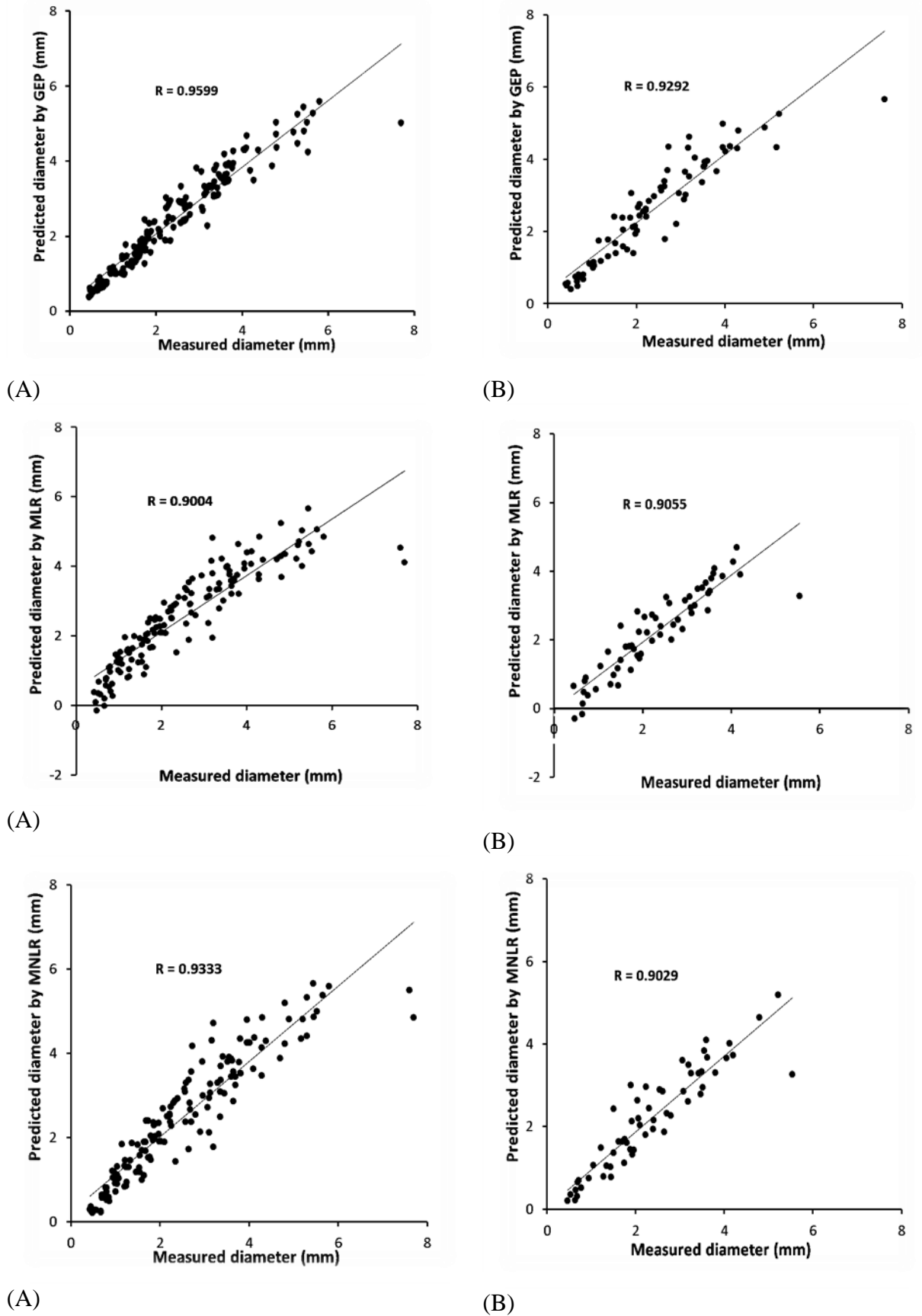
Figure 6. Scatter plot between measured average drop size and estimated by GEP, MLR and MNL models, Train data (A) and Test data (B)
