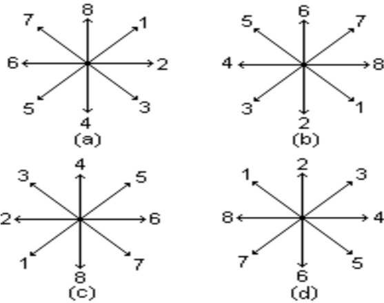
Fig.3. Directed vectors [11].
